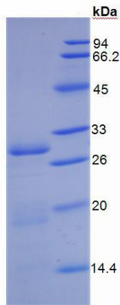
Figure 3. SDS-PAGE
