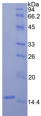
Figure 2. SDS-PAGE
