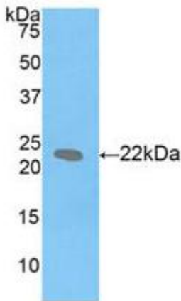
Figure 4. Western Blot
