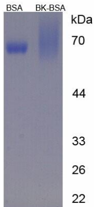
Figure 2. SDS-PAGE of BSA Conjugated BK
