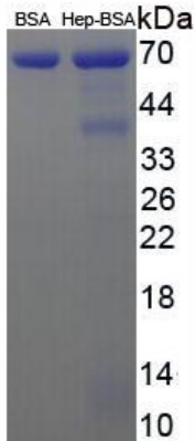
Figure 1. SDS-PAGE
