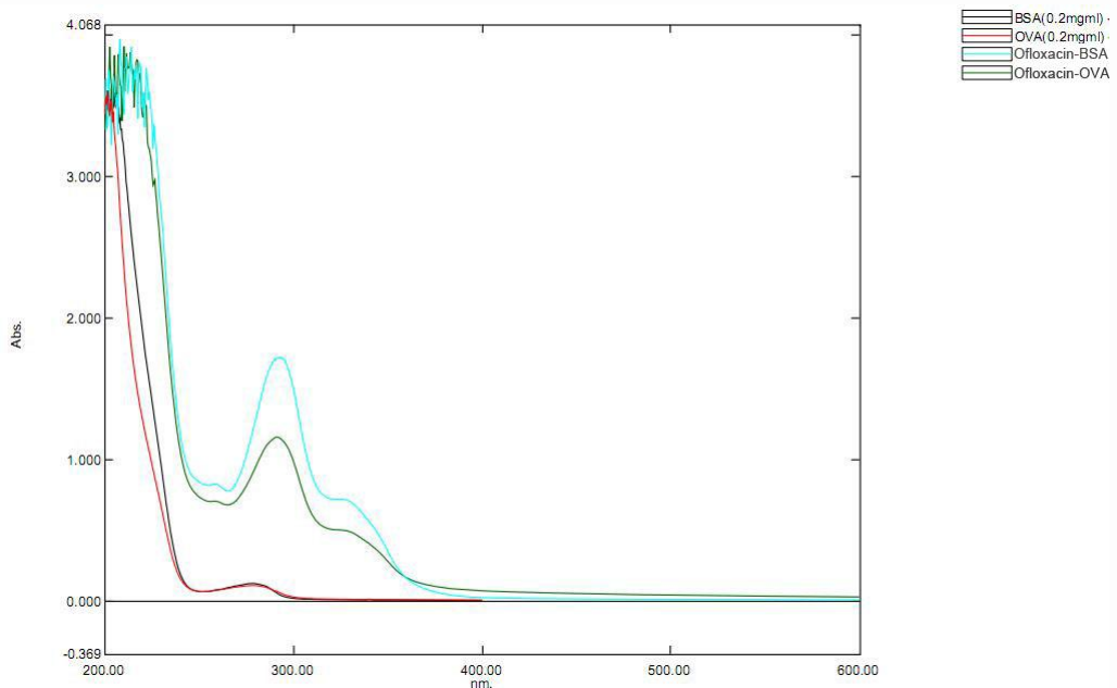
Figure 2. UV-spectrum
