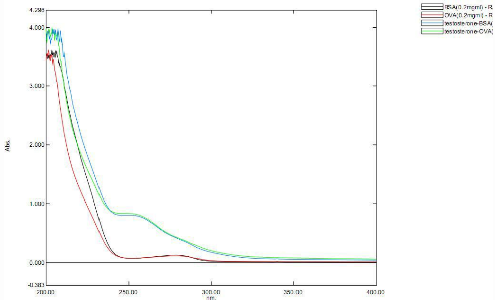
Figure 2. UV-spectrum
