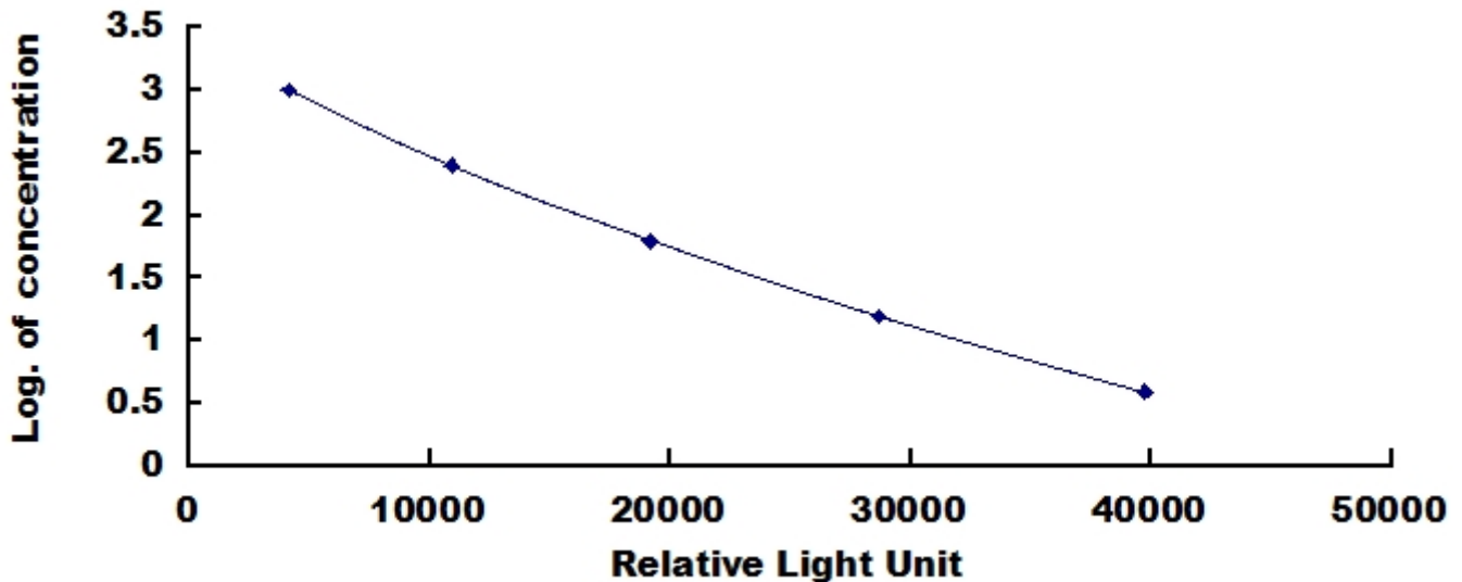
Typical Standard Curve for ATP CLIA.
