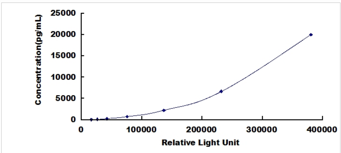
Typical Standard Curve for GDF2, Rat CLIA.
