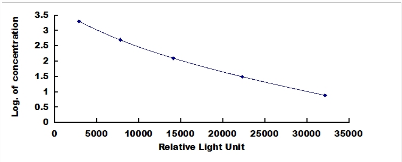
Typical Standard Curve for CGRP, Human CLIA.
