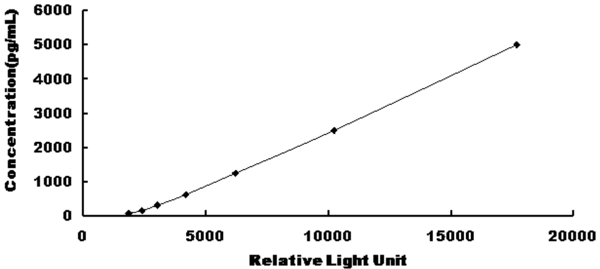
Typical Standard Curve for Human CCL3L1 CLIA.
