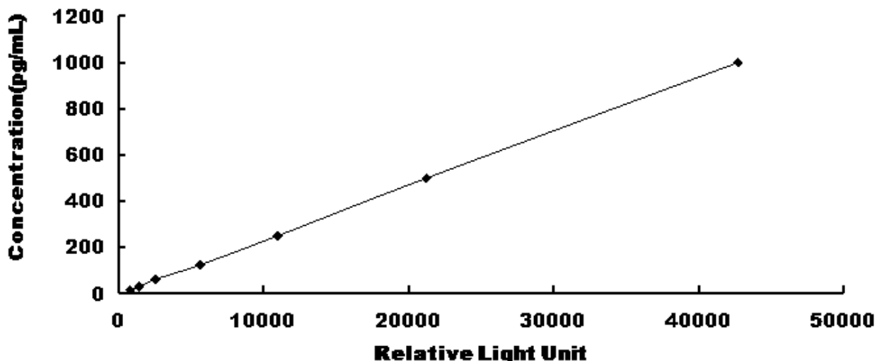
Typical Standard Curve for Rat GMCSF CLIA.
