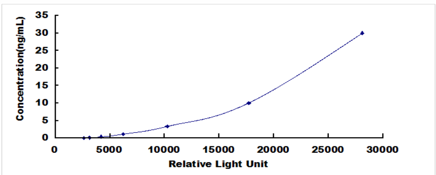
Typical Standard Curve for CYFRA21-1, Human CLIA.
