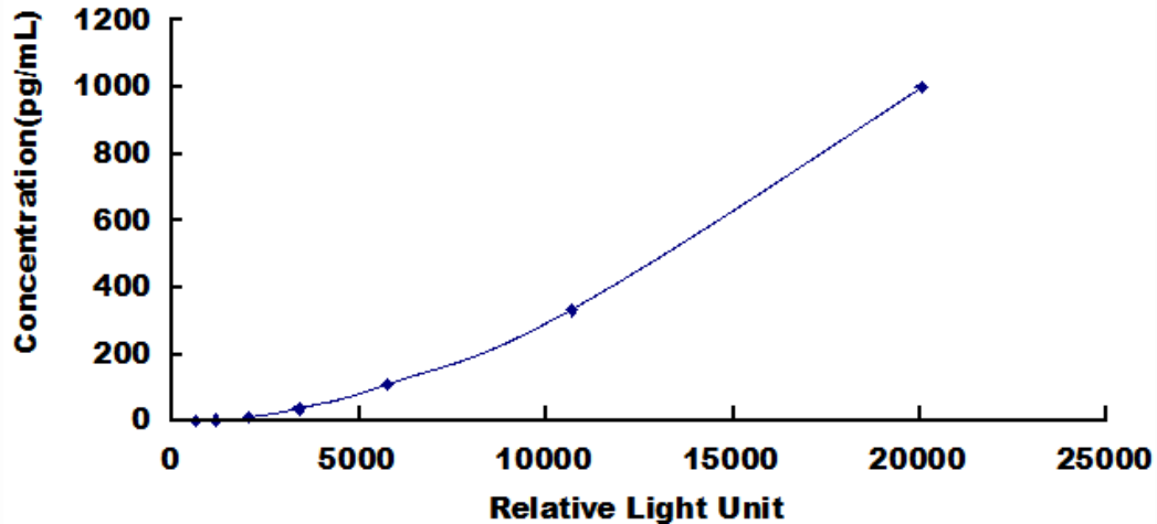
Typical Standard Curve for Erythropoietin, Mouse CLIA.
