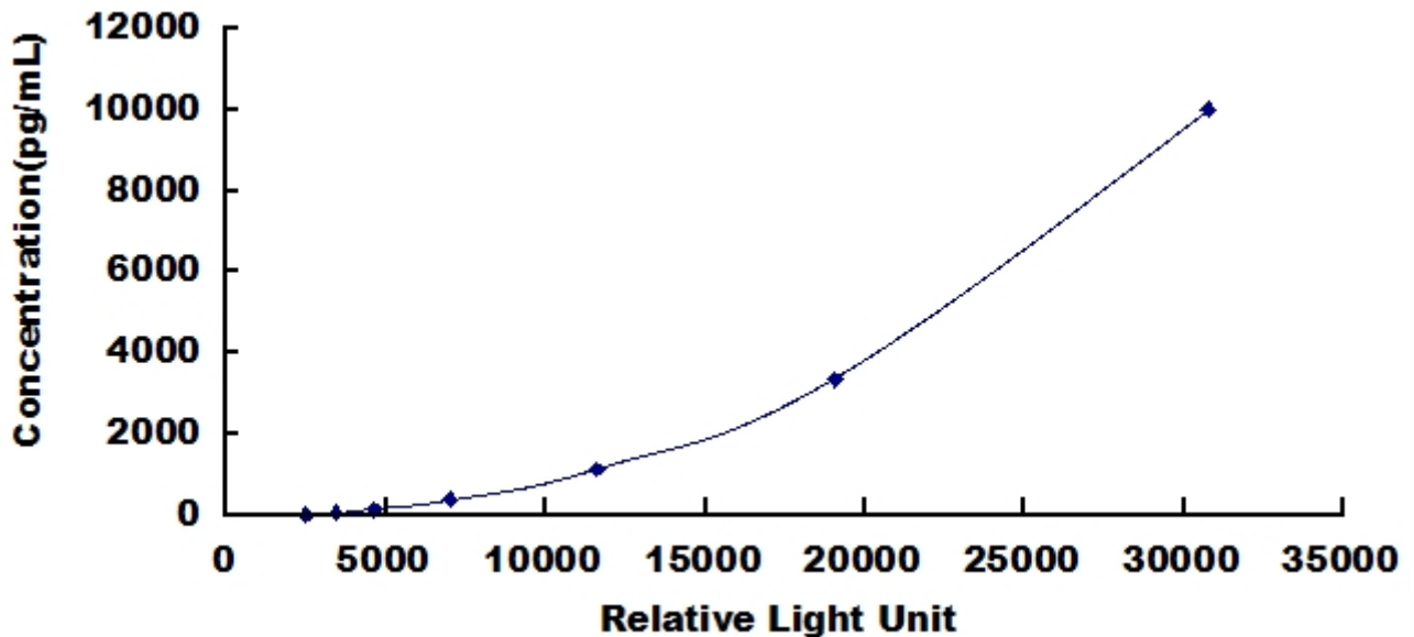
Typical Standard Curve for G6PC, Human CLIA.
