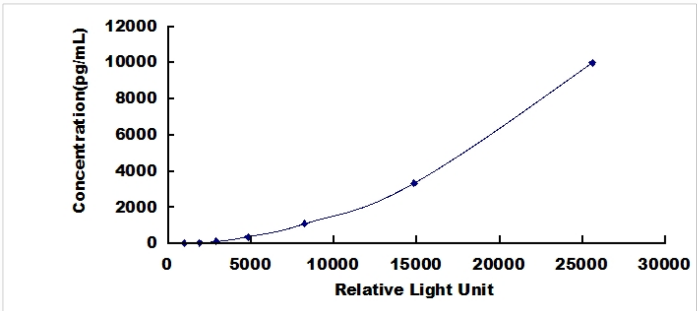
Typical Standard Curve for Hemopexin, Human CLIA.
