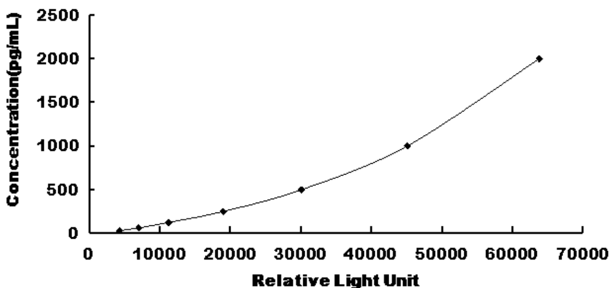
Typical Standard Curve for Human HBEGF CLIA.
