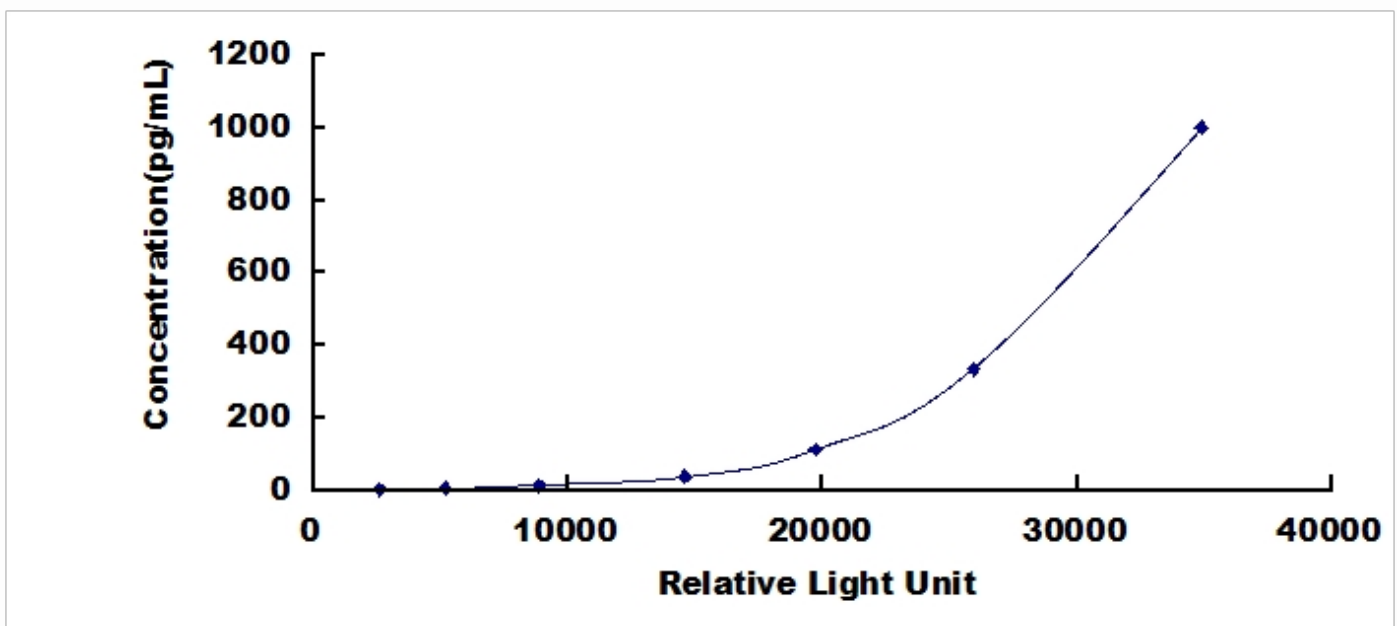
Typical Standard Curve for IL19, Human CLIA.
