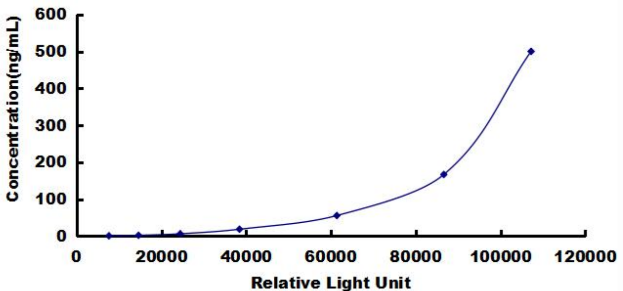
Typical Standard Curve for LDH, Mouse CLIA.
