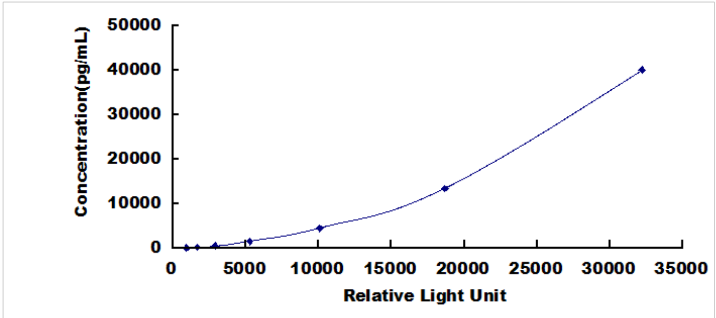
Typical Standard Curve for MMP13, Human CLIA.
