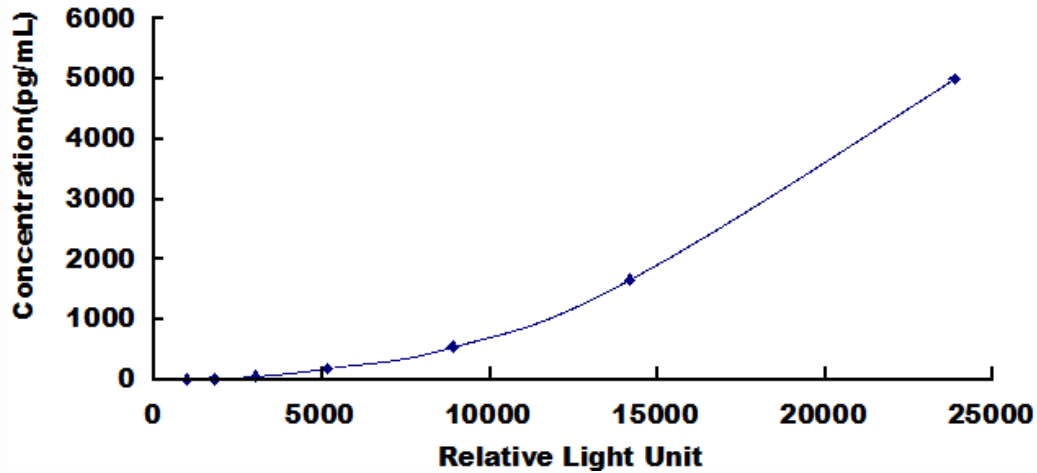
Typical Standard Curve for Procalcitonin, Human CLIA.
