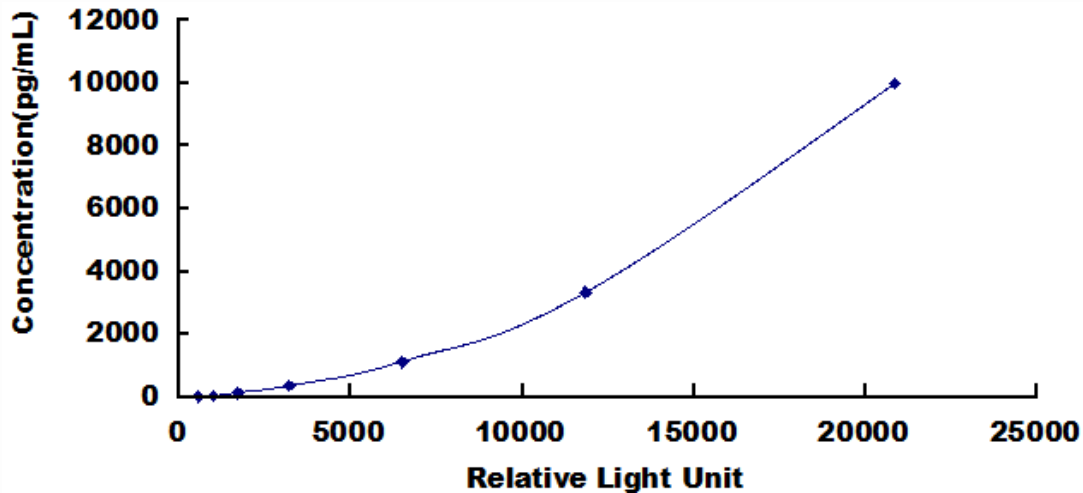
Typical Standard Curve for RANTES, Mouse CLIA.
