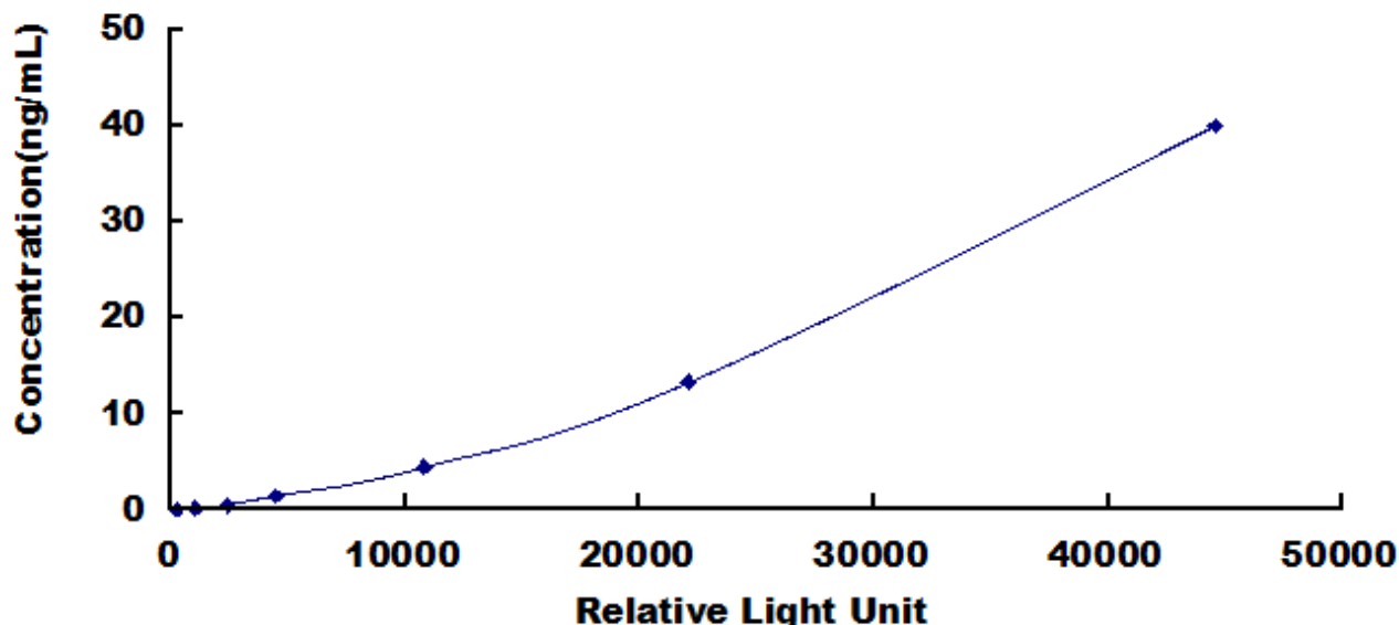
Typical Standard Curve for TFPI, Human CLIA.
