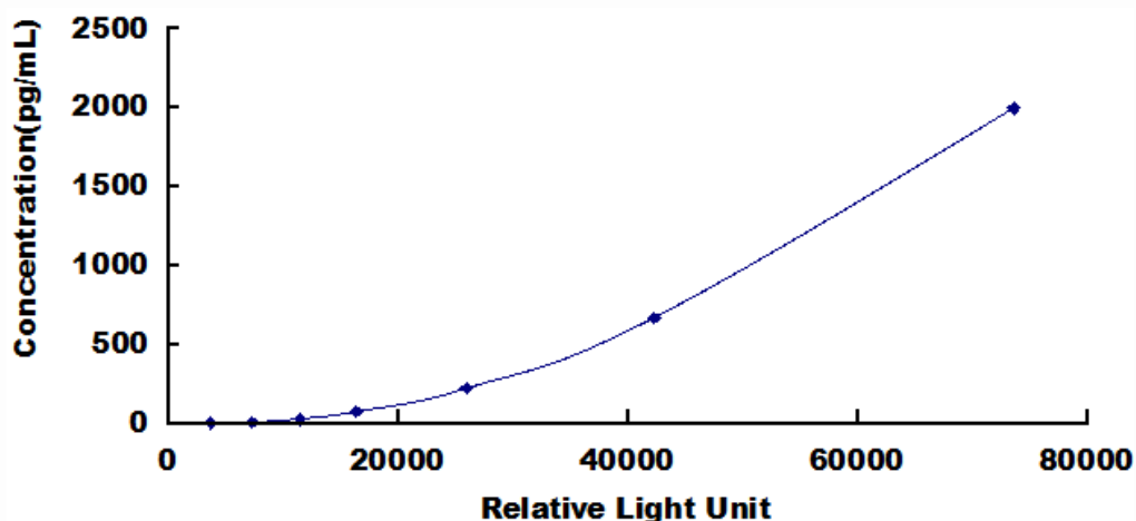
Typical Standard Curve for TGFb1, Human CLIA.
