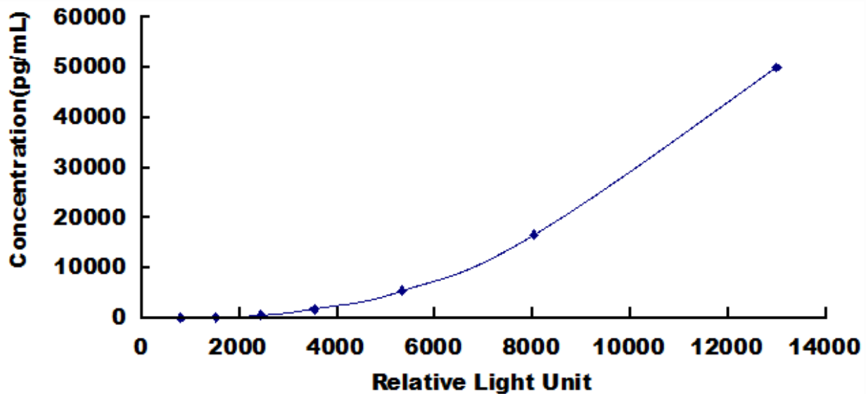
Typical Standard Curve for VCAM1, Mouse CLIA.
