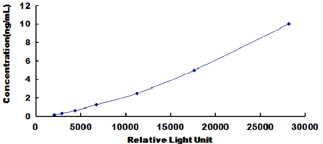
Typical Standard Curve for Human XIAP CLIA.
