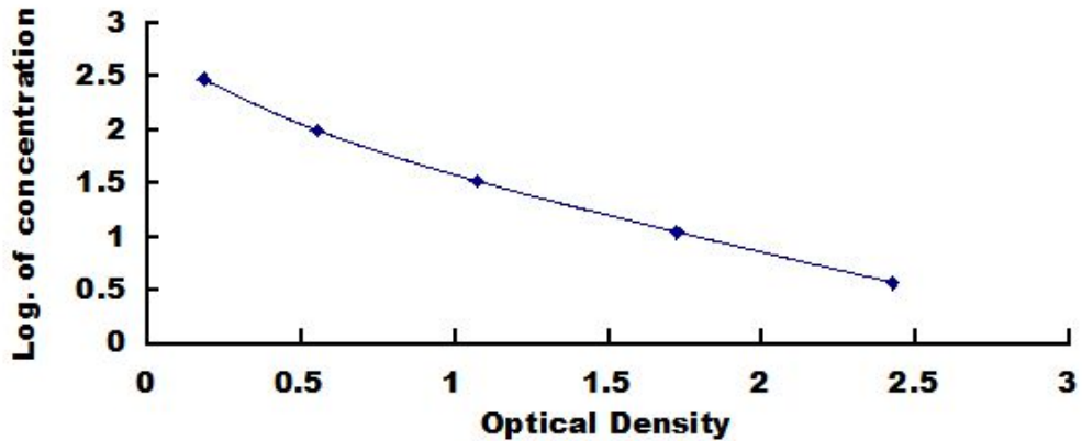
Typical Standard Curve of ELISA kit for Rat, NPY.
