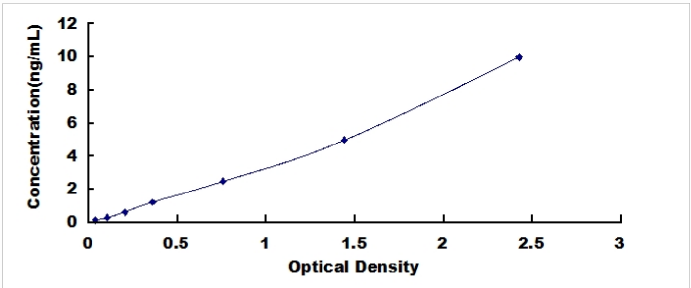
Typical Standard Curve for Androgen Receptor, Rat ELISA.
