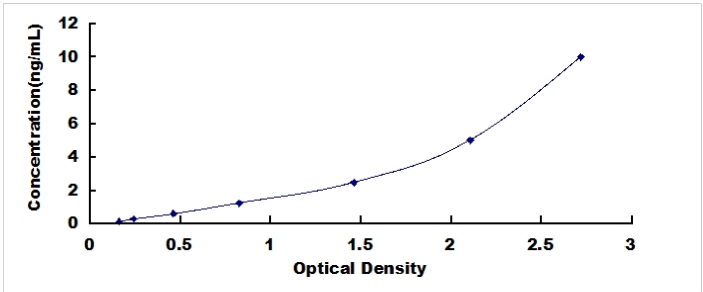
Typical Standard Curve for ANTXR1, Human ELISA.
