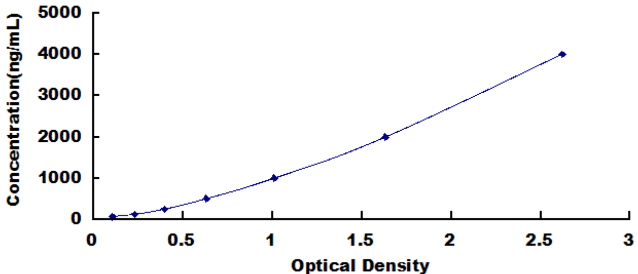
Typical Standard Curve for APOB, Mouse ELISA.
