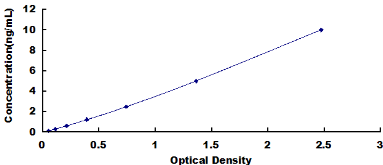
Typical Standard Curve for AIRE, Human ELISA.
