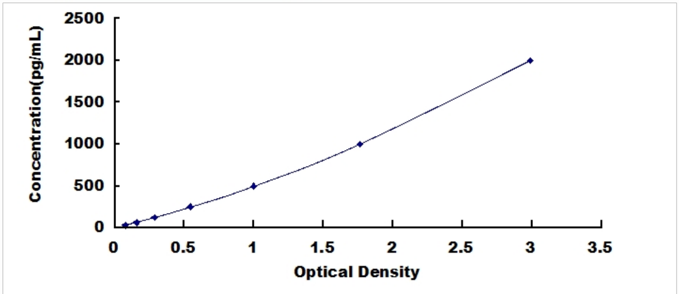
Typical Standard Curve for ATG12, Mouse ELISA.
