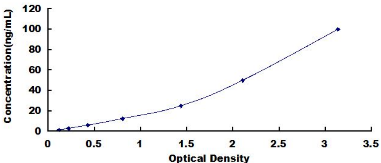
Typical Standard Curve for C1QTNF1, Human ELISA.
