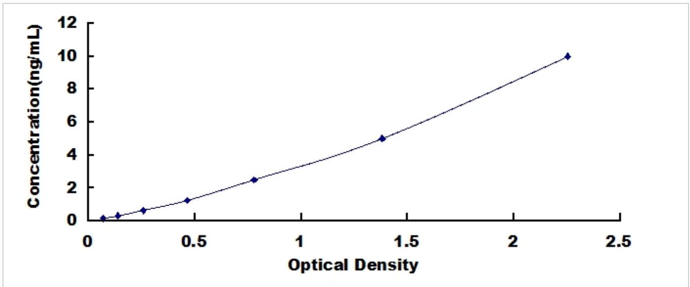
Typical Standard Curve for COMMD5, Human ELISA.
