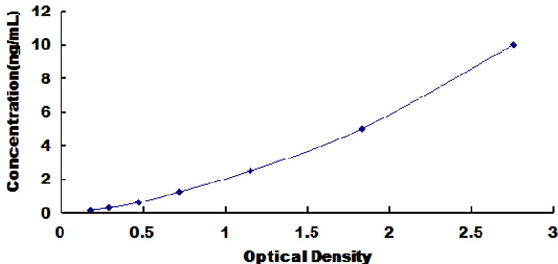
Typical Standard Curve for COMT, Mouse ELISA.
