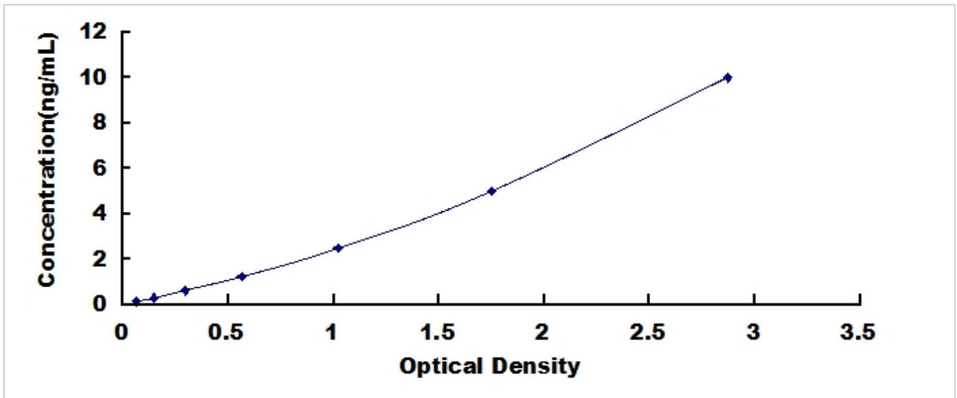
Typical Standard Curve for CETN1, Human ELISA.
