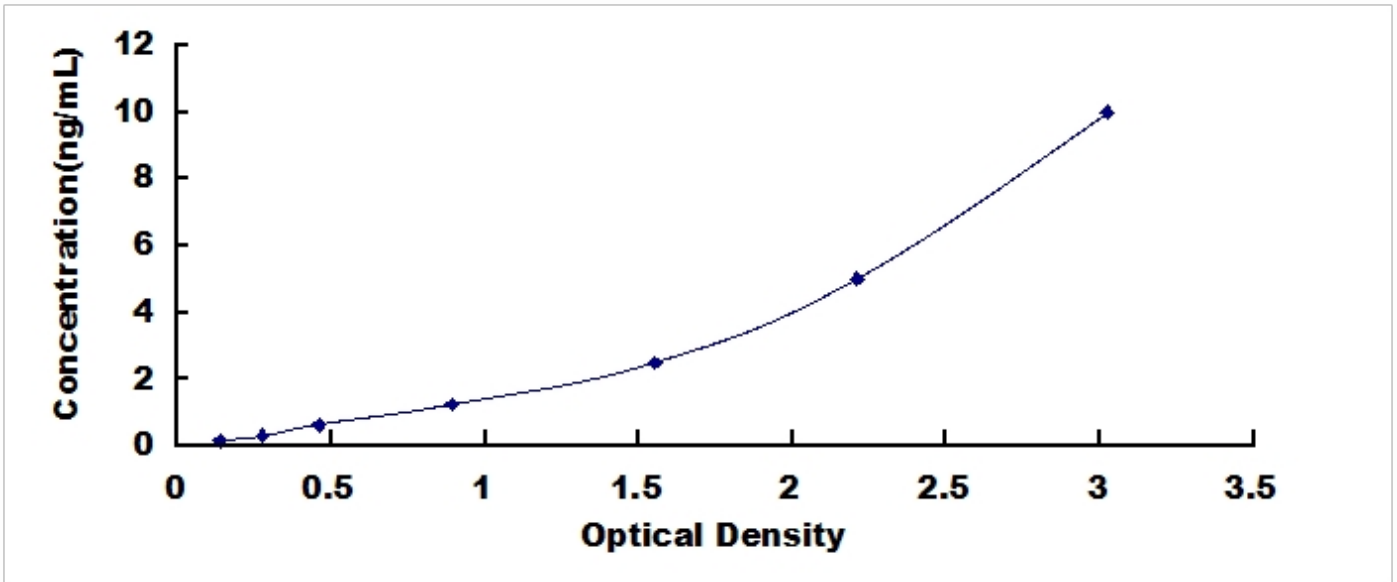
Typical Standard Curve for CCR4, Human ELISA.
