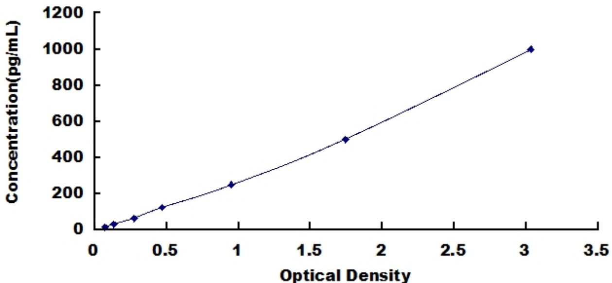
Typical Standard Curve for CCR5, Human ELISA.
