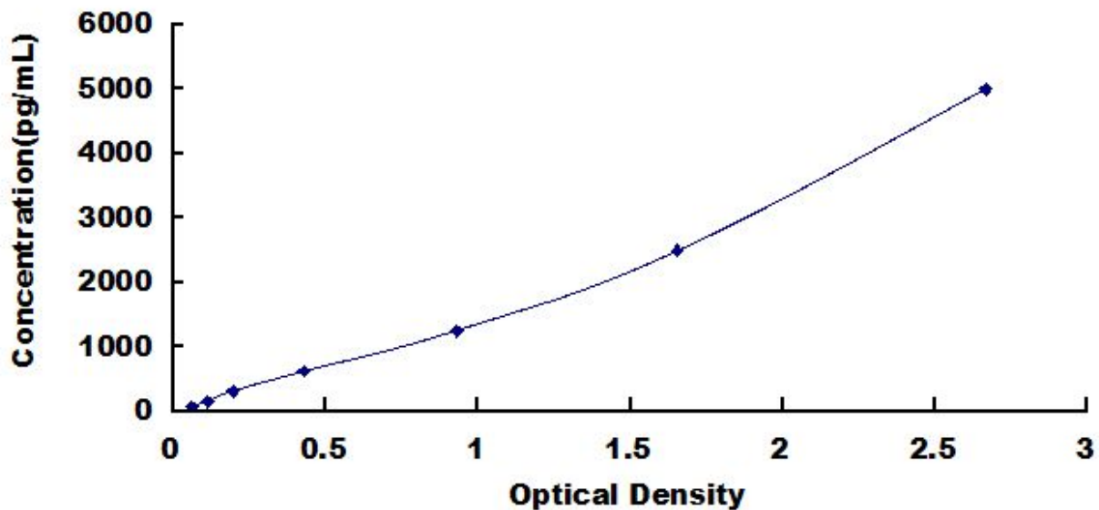
Typical Standard Curve for CR2, Human ELISA.
