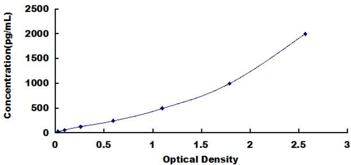
Typical Standard Curve for CTLA4, Human ELISA.
