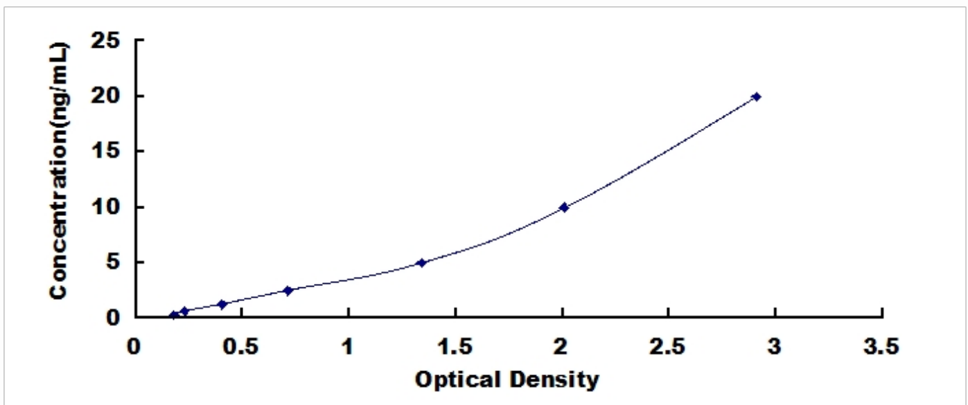
Typical Standard Curve for DEFa1, Human ELISA.
