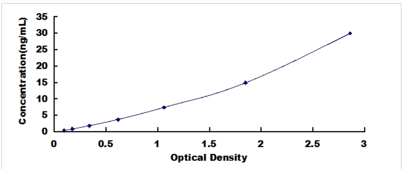
Typical Standard Curve for DEFa3, Human ELISA.
