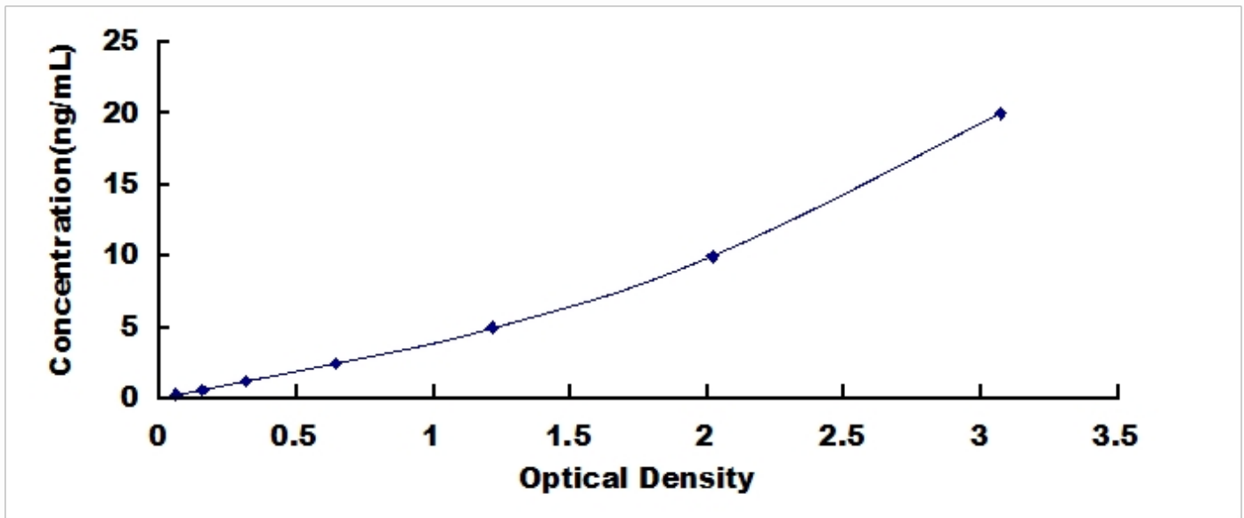
Typical Standard Curve for EP300, Rat ELISA.
