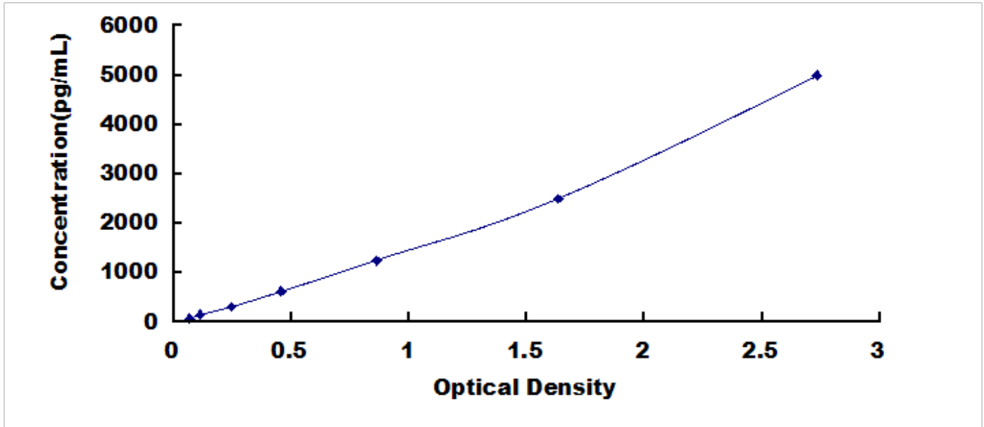
Typical Standard Curve for NNE, Mouse ELISA.
