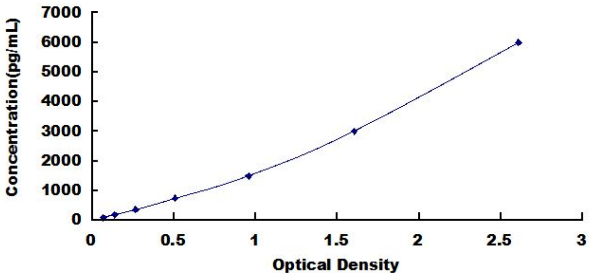
Typical Standard Curve for Erythropoietin, Rat ELISA.
