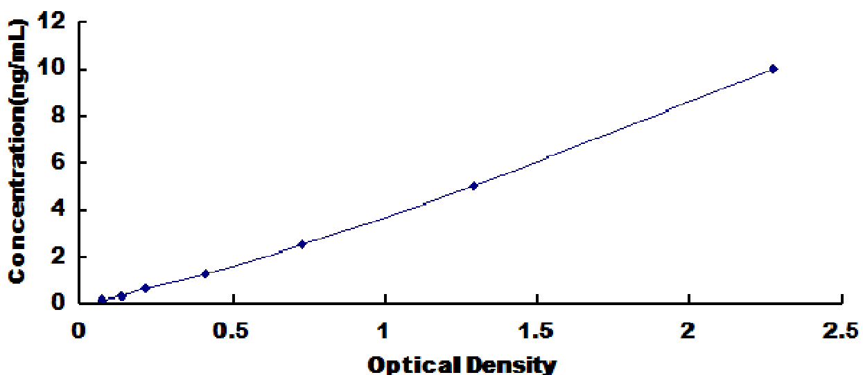
Typical Standard Curve for FBXO32, Human ELISA.
