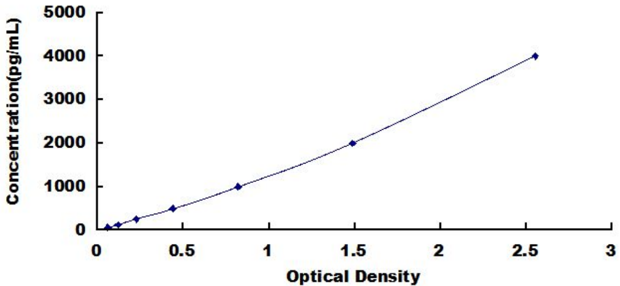
Typical Standard Curve for FADS1, Rat ELISA.
