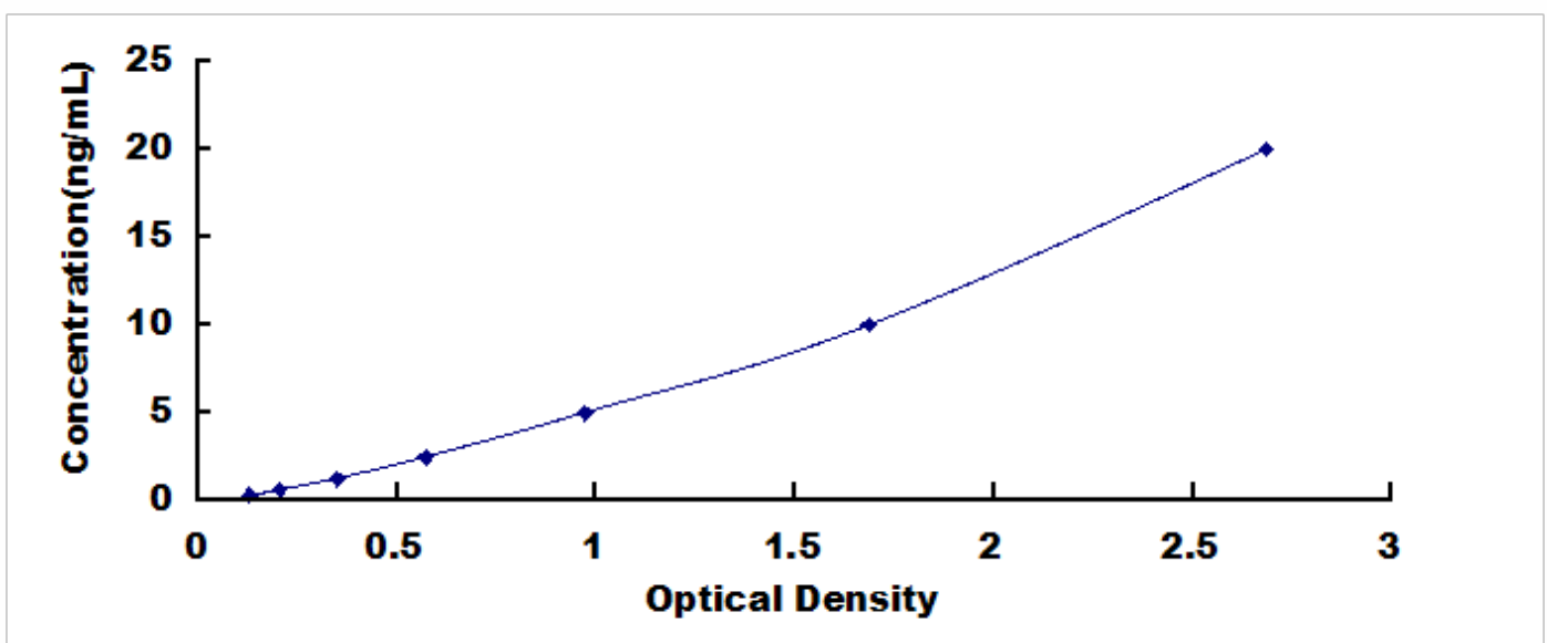
Typical Standard Curve for FGL2, Mouse ELISA.
