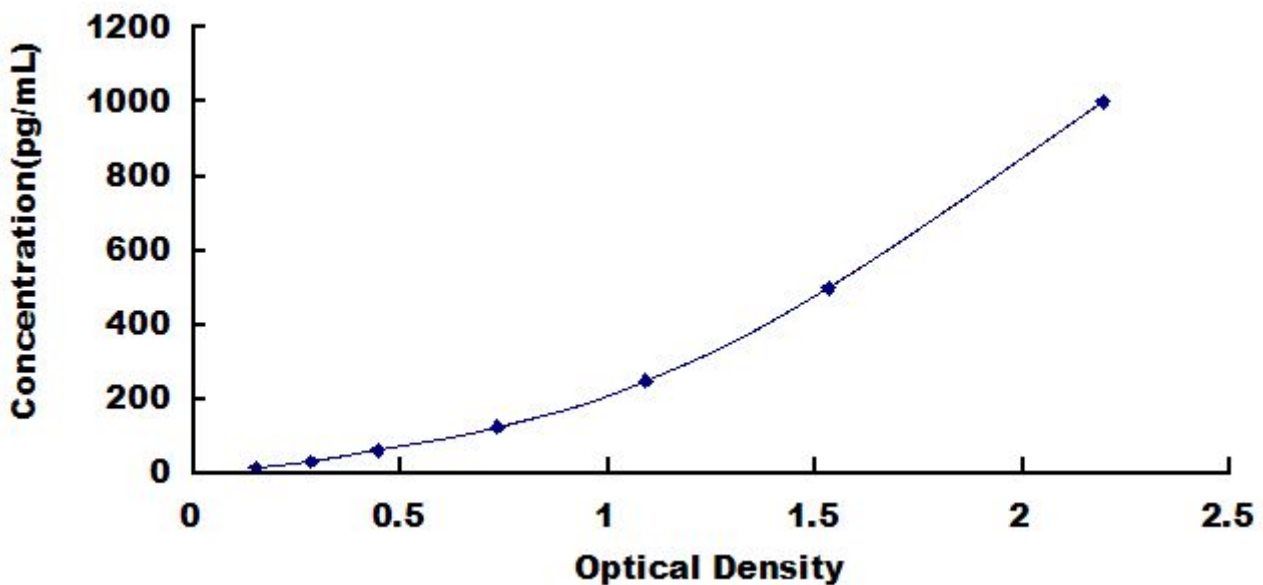
Typical Standard Curve for FGF21, Porcine ELISA.
