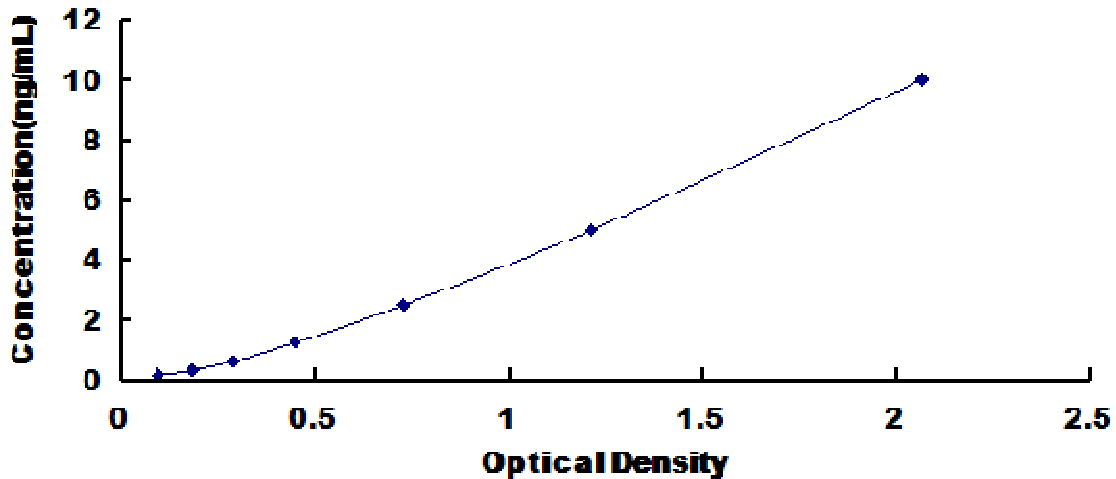
Typical Standard Curve for FFAR2, Mouse ELISA.
